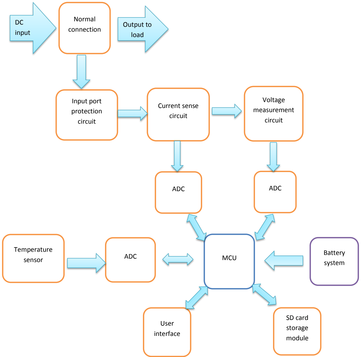
Figure 2: System Block Diagram
